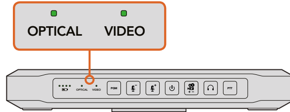
When a valid video signal is detected via SDI or HDMI, you'll see ATEM Camera Converter's 'video' status indicator illuminated. The 'optical' indicator will illuminate when a valid SDI signal is detected via the optical fiber input.
