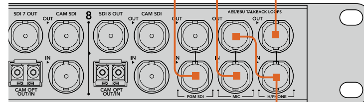
ATEM Talkback Converter 4K
